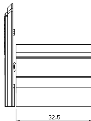
GUI114 (GUI007) p/ perfis VT-245/280
